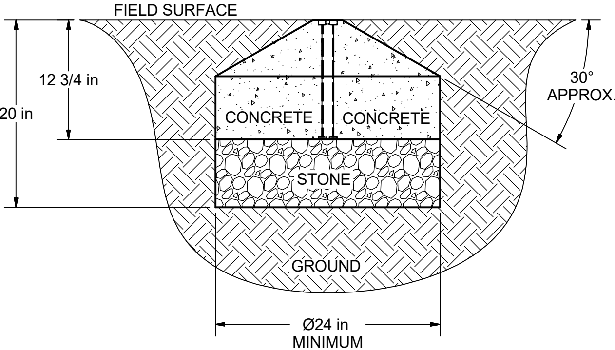
FOOTING DETAILS (4 PLACES)
