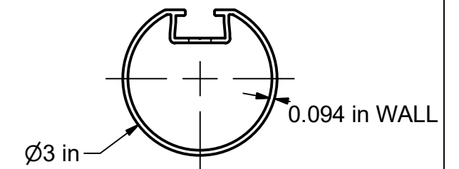
CROSSBAR MATERIAL - ALUMINUM
