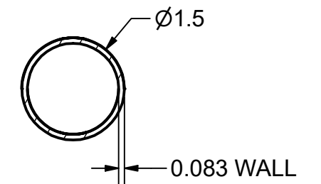
SHELTER BOW MATERIAL - ALUMINUM
