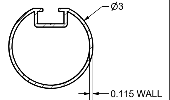
SHELTER FRAME MATERIAL - ALUMINUM
