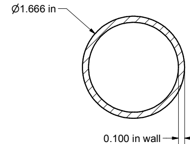
CORNER POLE AND GROUND SLEEVE MATERIAL - HIGH IMPACT PVC
