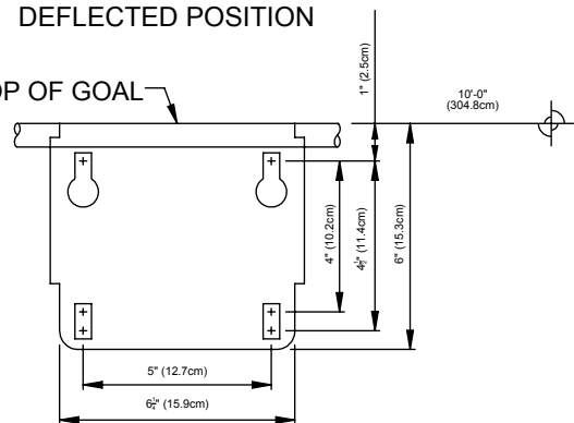
GOAL MOUNTING PLATE DETAIL (VIEW FROM BACKSIDE)
