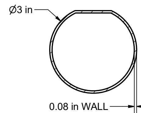
GOAL FRAME MATERIAL - ALUMINUM
