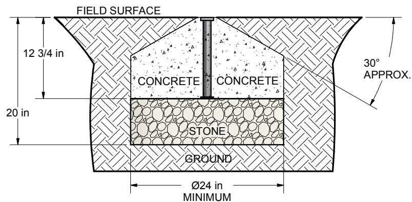
FOOTING DETAIL (4 PLACES)
