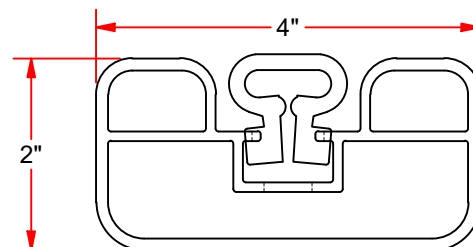
CHANNEL w/ NET CLIP
