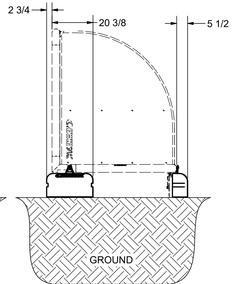
SIDE VIEW ATTACHED TO SHELTER
