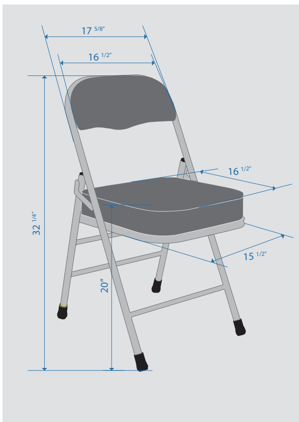
ISOMETRIC VIEW
