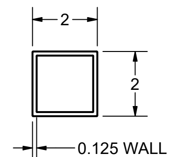
SEAT FRAMES MATERIAL - ALUMINUM
