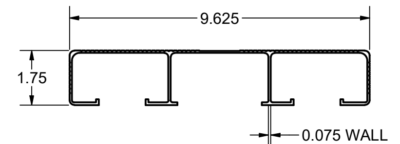
SHELF BENCH PLANK MATERIAL - ALUMINUM
