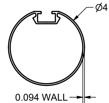
SHELTER FRAME MATERIAL - ALUMINUM
