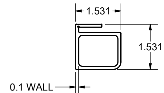
PANEL FRAMES MATERIAL - ALUMINUM
