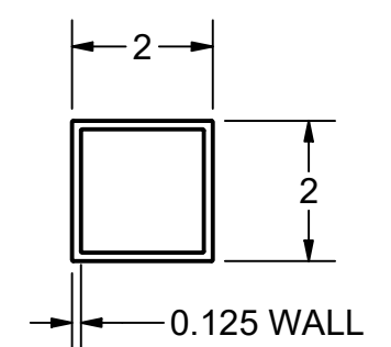
SEAT FRAMES MATERIAL - ALUMINUM
