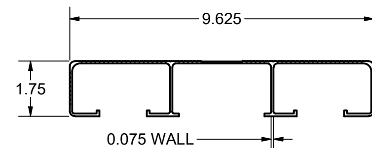
SHELF BENCH PLANK MATERIAL - ALUMINUM
