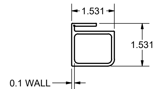
PANEL FRAMES MATERIAL - ALUMINUM
