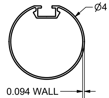
SHELTER FRAME MATERIAL - ALUMINUM
