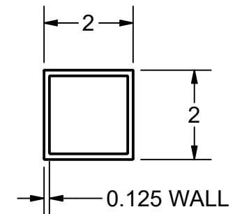
SEAT FRAMES MATERIAL - ALUMINUM
