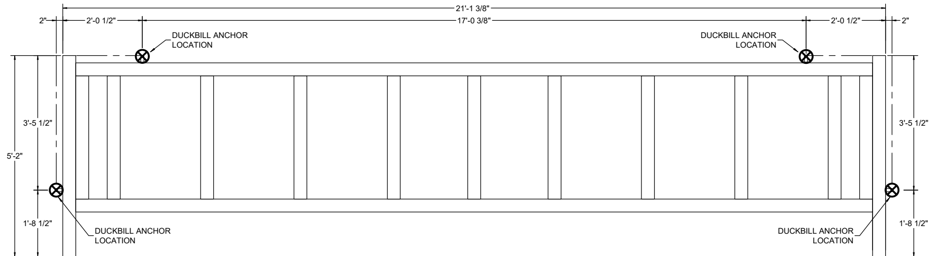
TOP VIEW OF SHELTER BASE FRAME
