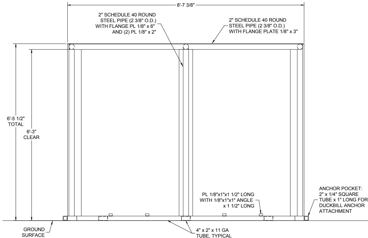
FRONT VIEW OF SHELTER
