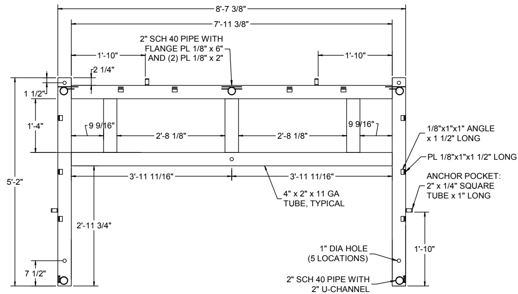
TOP VIEW OF BASE FRAME
