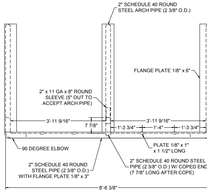
TOP VIEW OF ARCHES AND CROSSBAR
