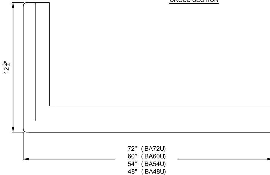
CROSS SECTION
