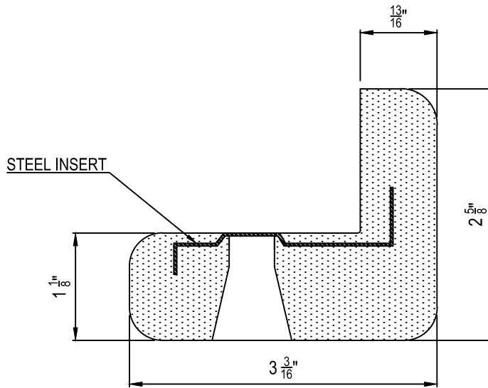
CROSS SECTION
