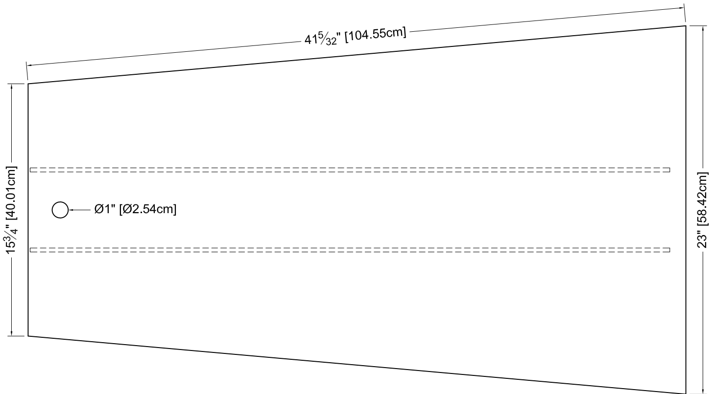
Top View of 50202 Lid
