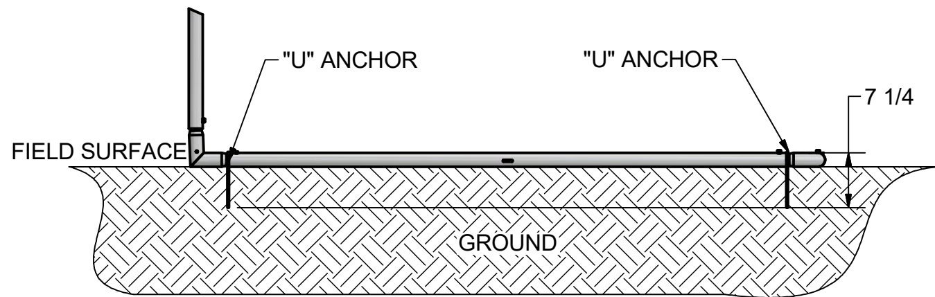
ANCHOR DETAILS (4 PLACES)
