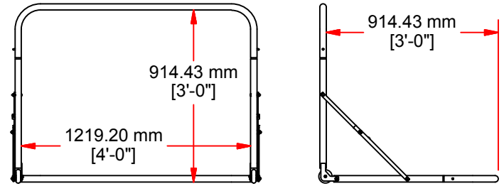
OVERALL DIMENSIONS
