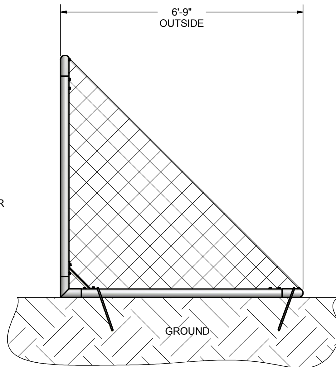
SIDE VIEW
