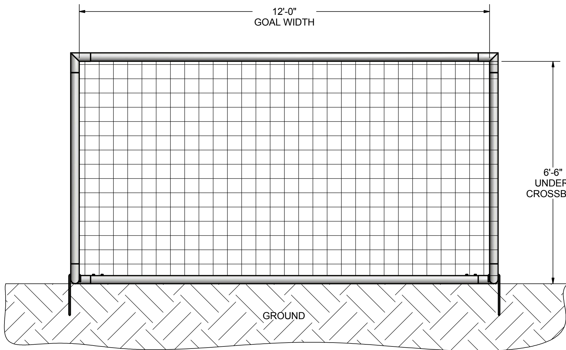
FRONT VIEW
